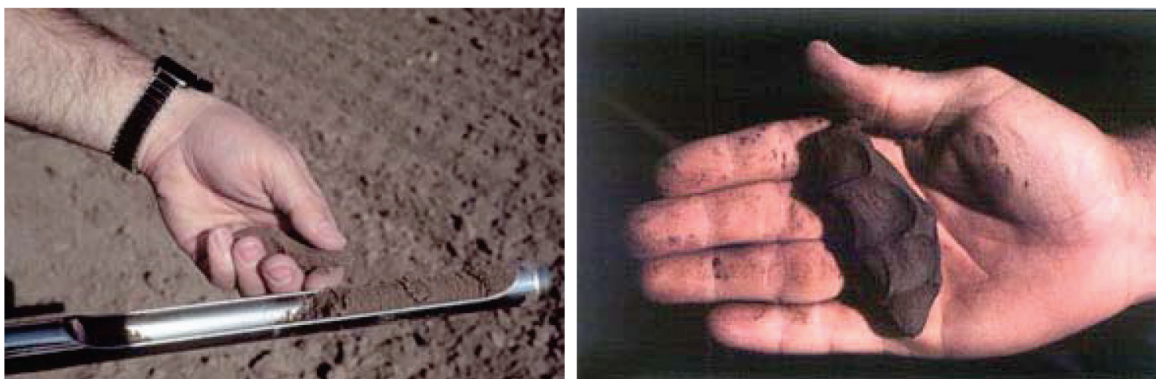
Figure J-3. Sampling and evaluation techniques for the feel method of soil water monitoring.
