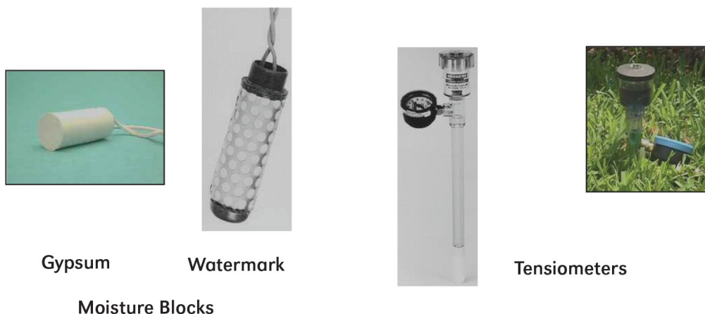
Figure J-4. Methods of measuring the soil matric potential.
