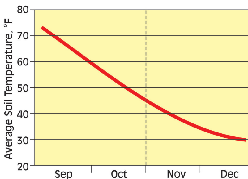
Figure G-4. Average soil temperature in the fall at Clay Center, NE.
