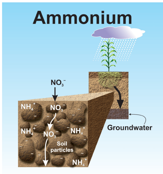
Figure G-5. Depiction of the attachment of positively charged ammonium molecules to negatively charged soil particles, which prevents leaching of N in the ammonium form while allowing leaching in the nitrate form.
